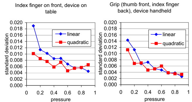
Figure 2. Standard deviation for different pressure levels during 3s intervals. Variability is high for low pressure levels. The FSRs are attached to voltage dividers.
