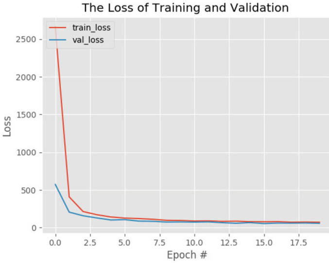
Fig. 7.6 Loss function of YOLOv3 training
