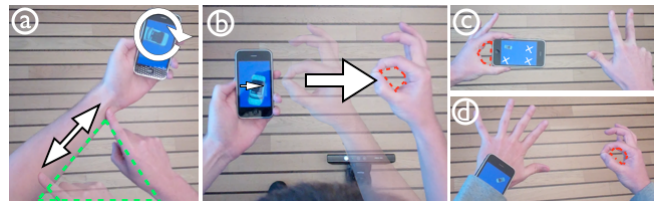
Figure 7: 3D control on mobile devices. (a) Moving the finger along the arm (modifying the shape of the triangle) rotates the 3D object. (b) x, y and z translation with 3D radial gestures. (c) The user chooses a predefined control with a finger-count gesture (3 fingers on the right hand + a pinch formed by the left hand and the device). (d) Finger-count gestures to select commands on a watch (simulated by an iPhone on the wrist).
